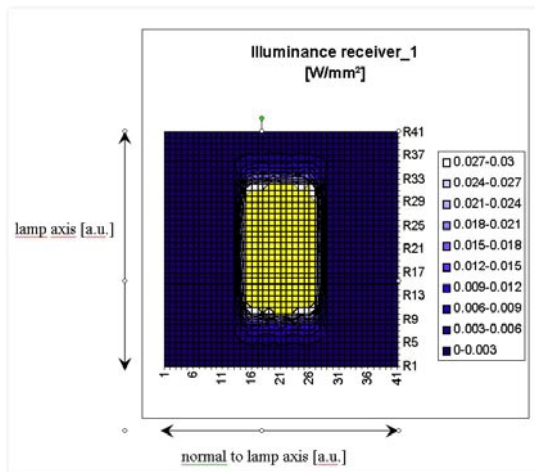
Contour “maps” of the UV lamp output aid in the development of curing simulations. The output can be modeled into a robot tool for path programming.
