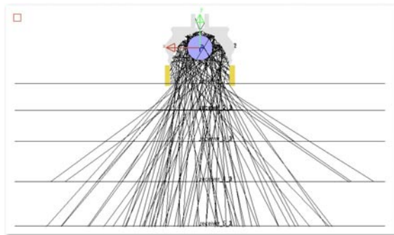
Ray tracing of the IST robot lamp. Note that the reflector is optimized to provide uniformity at typical target distances.
