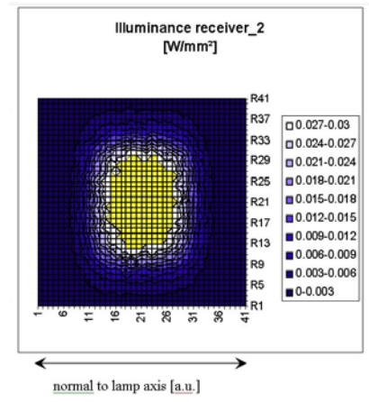
Contour “maps” of the UV lamp output aid in the development of curing simulations. The output can be modeled into a robot tool for path programming.
