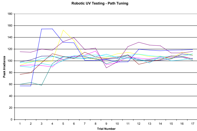
Fine tuning the path over the course of several runs to minimize variation in peak irradiance as measured on 10 different UV sensors.
