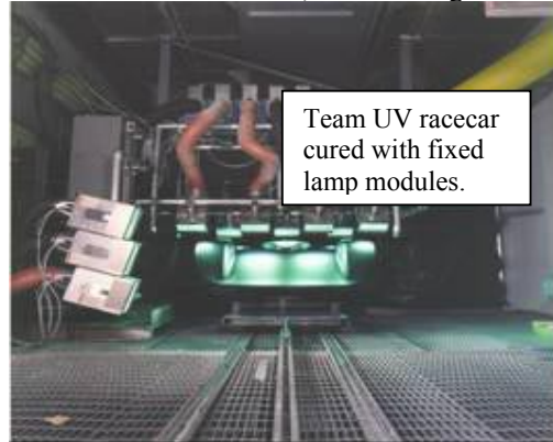
The Team UV racecar project used many fixed lamps to cure a small UV coated race car.
