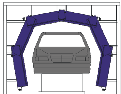
Using larger lamp lengths improves the cost and logistics of the fixed lamp approach but still presents geometry problems.
