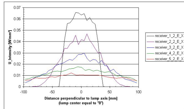
Profile of the robot lamps output at various distances from the center of the lamp axis.
