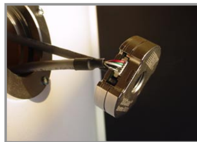
Close up view of one of the UV sensors implanted on the test surface and connected to a data acquisition module.
