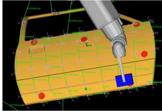
Development of the offline UV simulation software is a continuing effort to reduce setup time.
