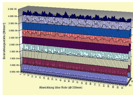
The resulting irradiation profile. The profile is not perfectly uniform because of various factors including; gaps between lamps, varying target distance along the lamp length and edge effects from each lamp.
